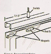
Figure 1. Recessed installation
